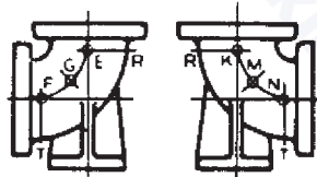
90° BASE ELBOW
