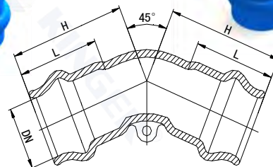
ELBOWS 45° SERIES-5250
