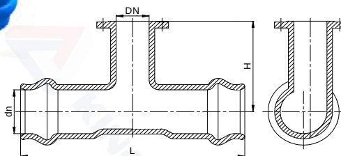
PVC double socket level invent tee with flanged branch
