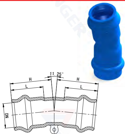
ELBOWS 11.25° SERIES-5200
