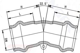
ELBOWS 22.5° SERIES-5225
