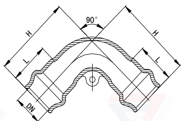
ELBOWS 90° SERIES-5175
