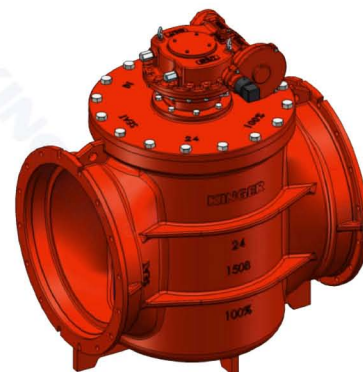
With Wrench Nut
