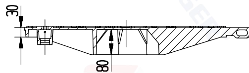
SECTION C-C
