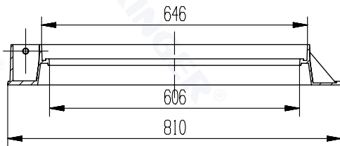
SECTION E-E
